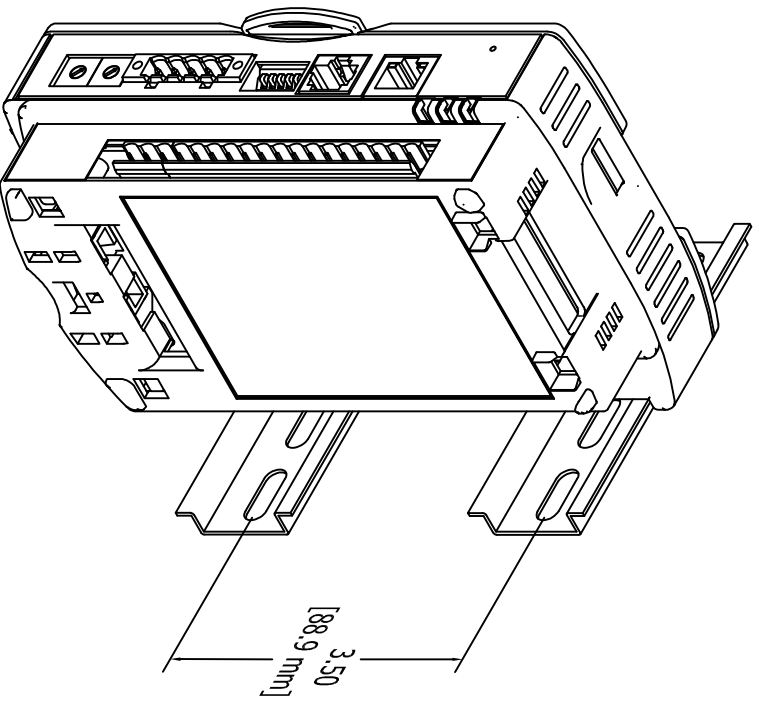
VERTICAL MOUNTING OPTION
